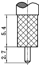
Recommended cable stripping dimensions
