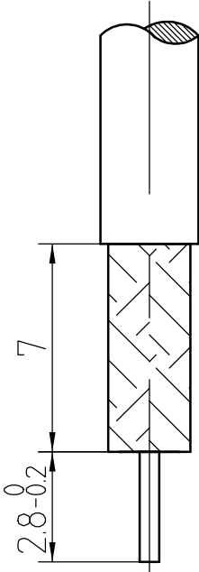
Recommended Cable Stripping Dimension
