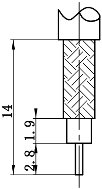
Cable Stripping Dimension
