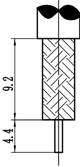
Recommended Cable Stripping Dimension
